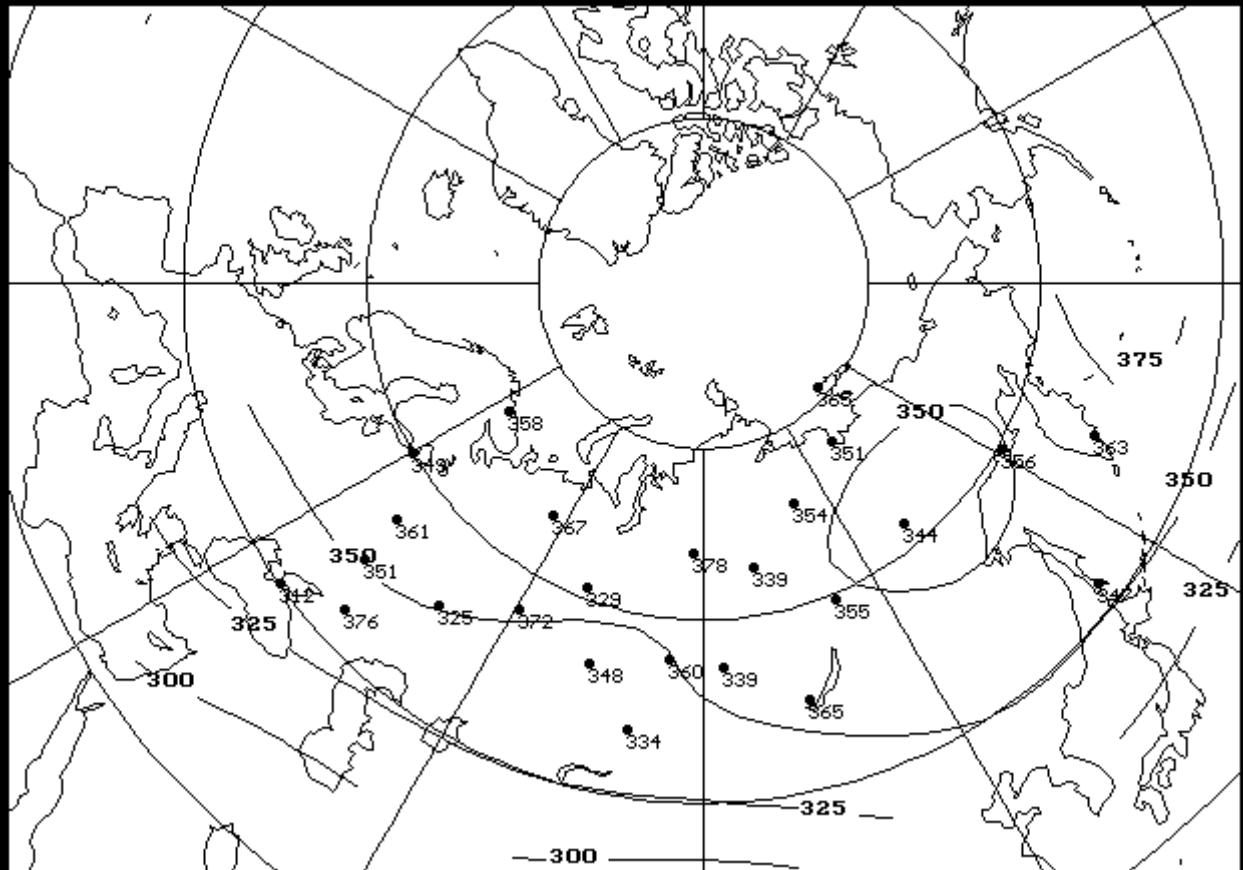
Total ozone (D.U.) for June 1, 2025 - June 30, 2025.
