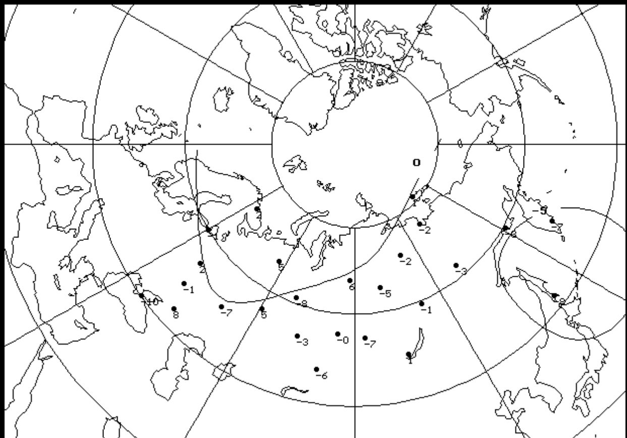
Deviations (%) for June 1, 2025 - June 30, 2025.
